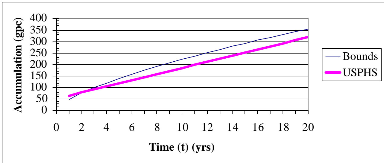
Figure 3: Rates of Septage ( sludge/scum ) accumulation (95 percent level of confidence)
