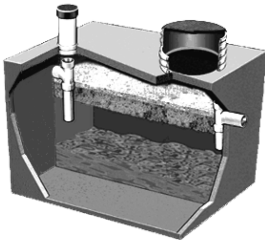
Figure 5: Typical Gravity Septic Tank (Single Compartment)
